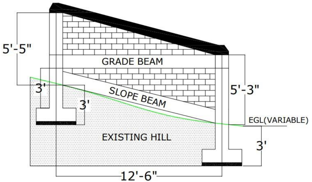
TYPICAL SECTION
