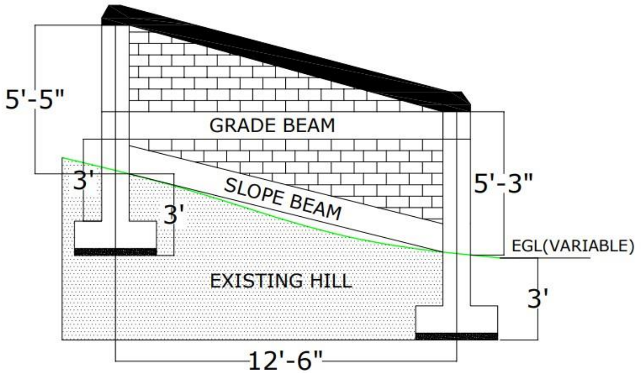
TYPICAL SECTION
