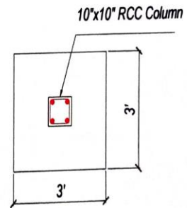
Boundary Column Plan
